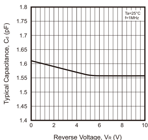
Fig.2 - Capacitance Characteristics
