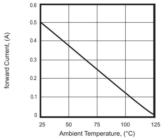
Fig.4 - Power Derating
