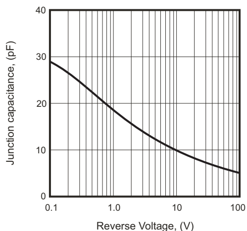
Fig.5 - Junction Capacitance
