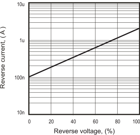
Fig. 3 - Reverse characteristics
