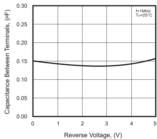
Fig.4 - Typical Capacitance Between Terminals Characteristics
