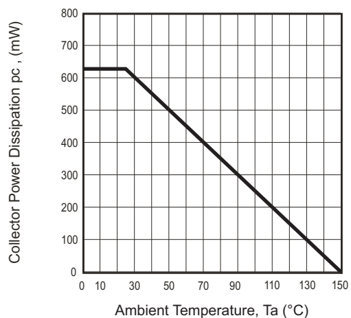
Fig.5 - P_C - T_a
