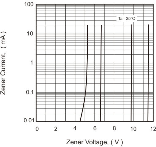
Fig.2- Zener Breakdown Characteristics
