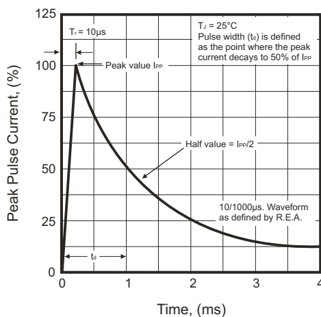
Fig.5 - Pulse Waveform
