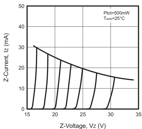
Fig.6 - Z-Current vs. Z-Voltage
