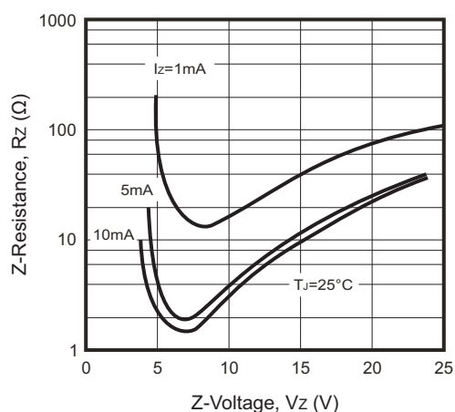
Fig.4 - Differential Z-Resistance vs. Z-Voltage
