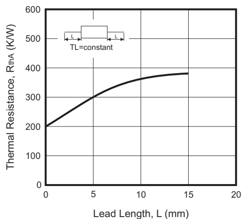
Fig.2 - Thermal Resistance vs. Lead Length
