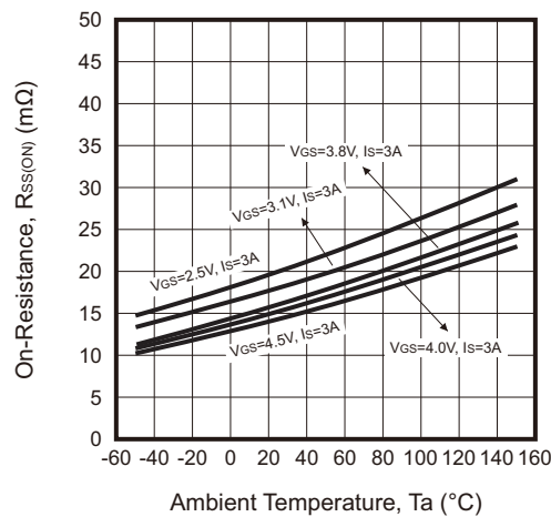
Fig.9 - R_{DS(ON)} — T_a
