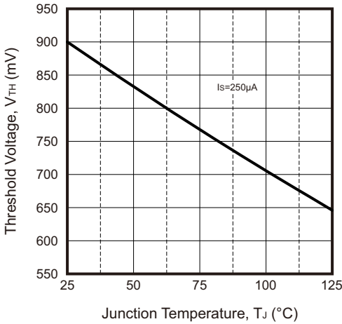
Fig.6 - Threshold Voltage
