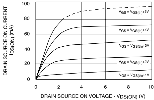
OUTPUT CHARACTERISTICS
