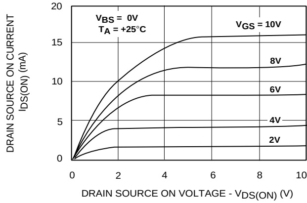
OUTPUT CHARACTERISTICS
