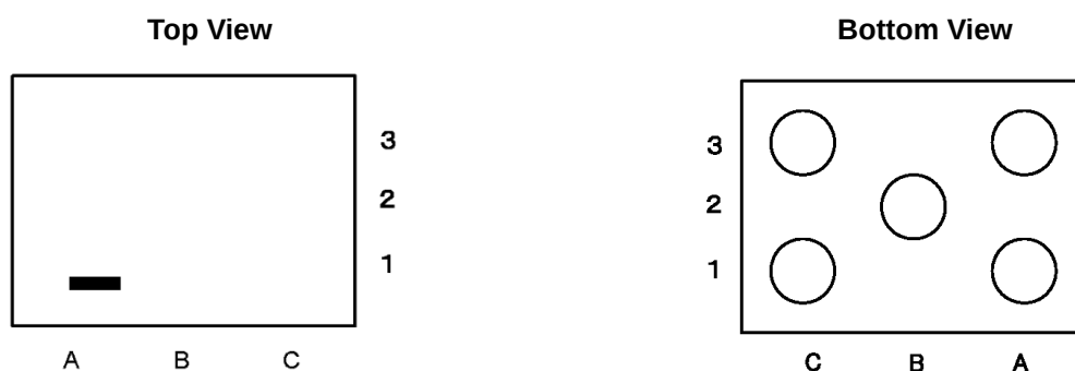
WLCSP-5-P1 Pin Configurations
