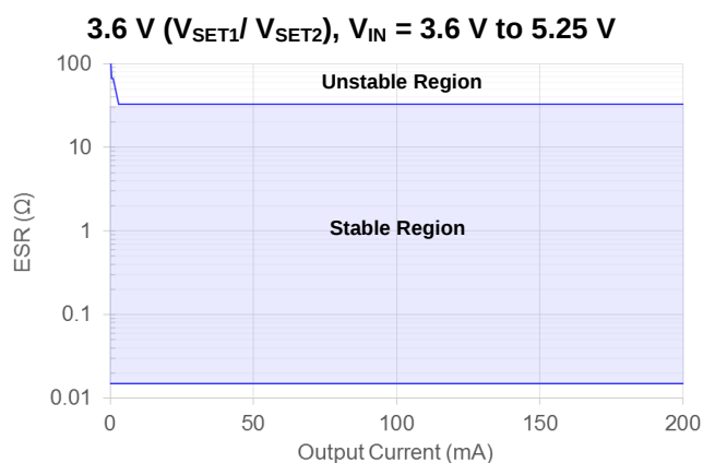
Fig. 4 Range of Stable ESR Values
