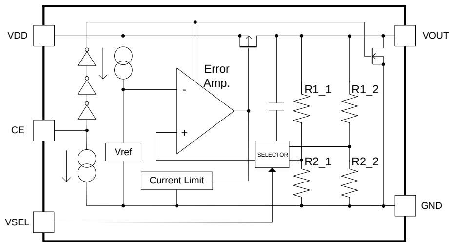
RP155Z Block Diagram
