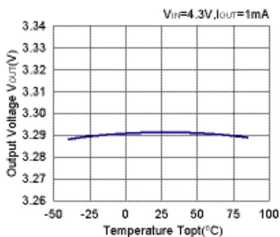
3.3V(VR1/VR2)
