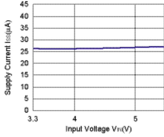
3.3V(VR1/VR2)
