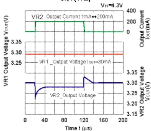
3.3V(VR2)
