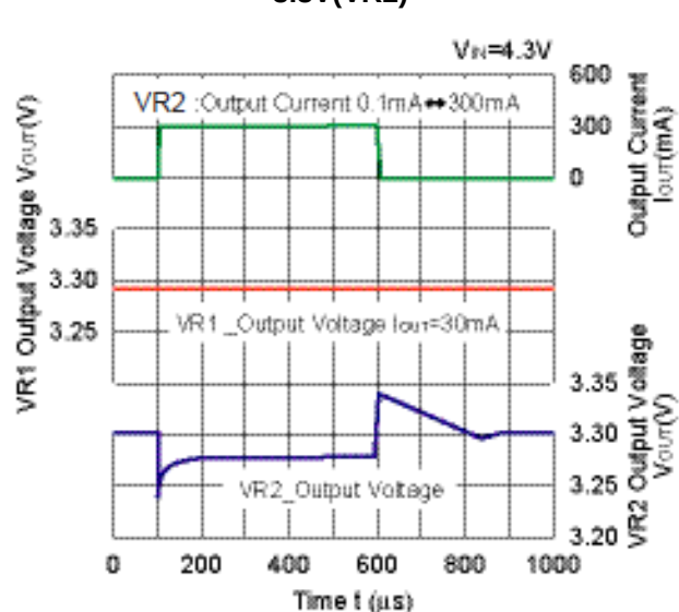
3.3V(VR2)
