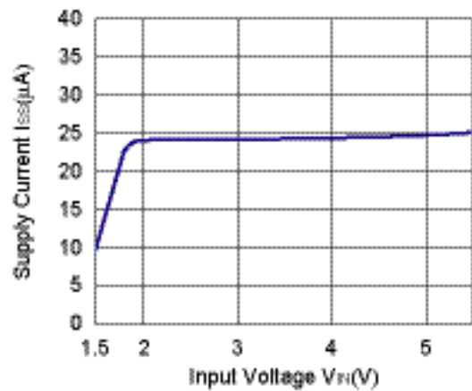
1.5V(VR1/VR2)
