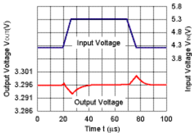
3.3V(VR1)
