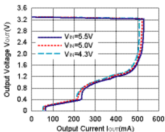
3.3V(VR1/VR2)
