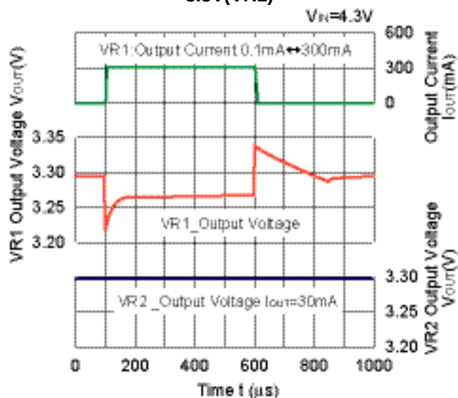
3.3V(VR1)
