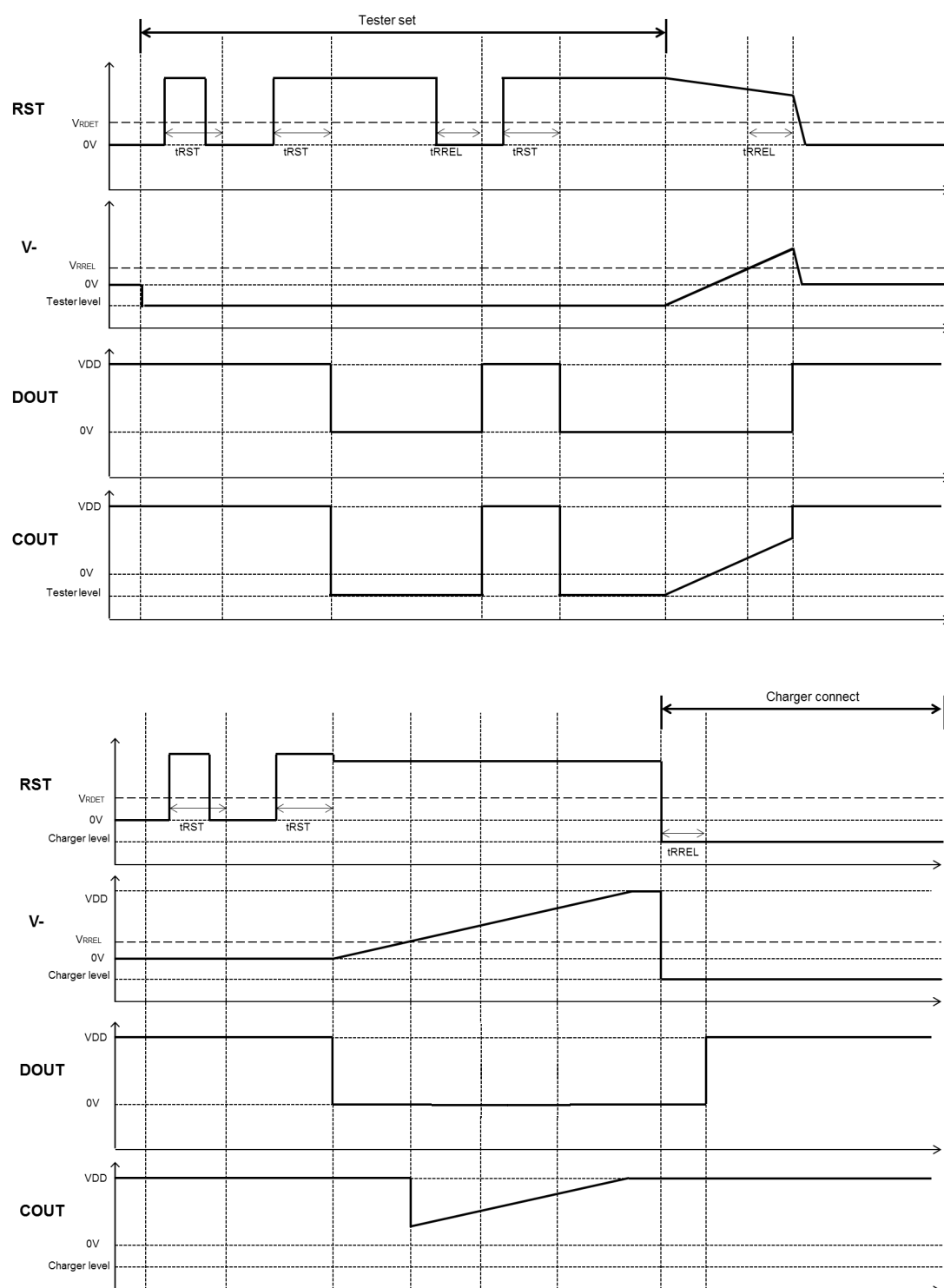
RST Pin Function (Forced-standby type) Timing Diagram
