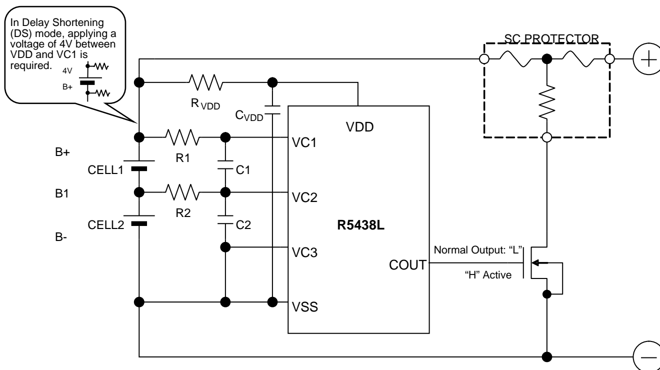
Typical Application Circuit for 2-cell Protection -1
