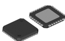
HQFN0808-28 8.8 x 8.8 x 0.95 (mm)
