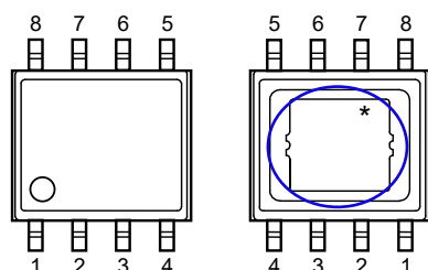
HSOP-8E Pin Configuration
