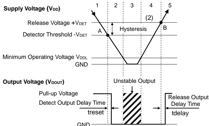
Operation Diagram
