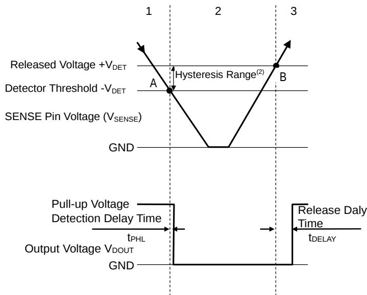
Diagram for R3121xxxE with External Capacitor
