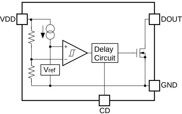
R3121NxxxA/R3121NxxxG
