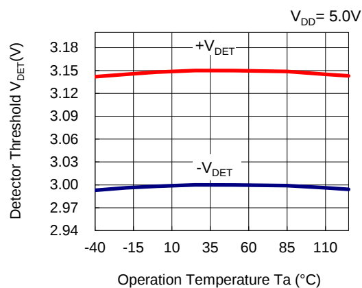
R3121N030E
