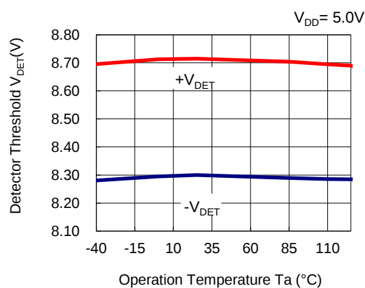
R3121N083E
