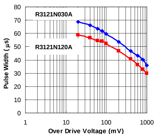
R3121NxxxA/G Pulse Width vs. Over Drive Voltage
