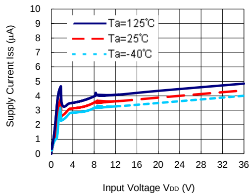
R3121N083A/G
