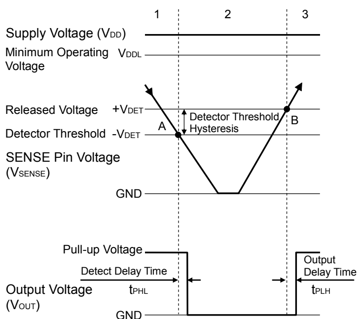
Operation Diagram
