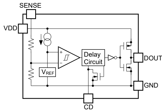
R3118xxxxC (CMOS Output) Block Diagram
