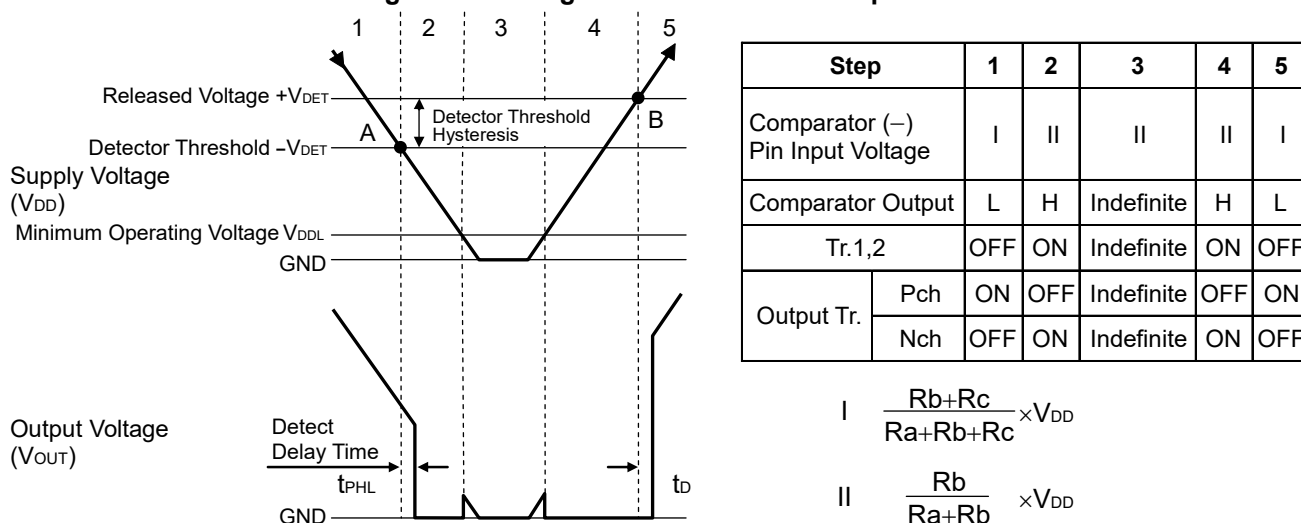
Fig. 2 Operation Diagram
