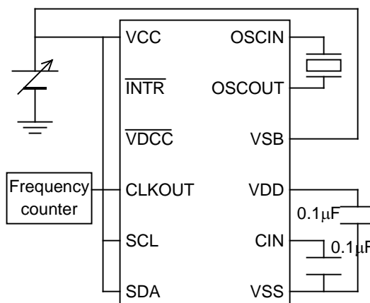
Test circuit
