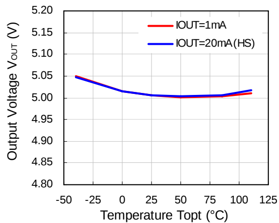
R1510S (VR=5.0V)
