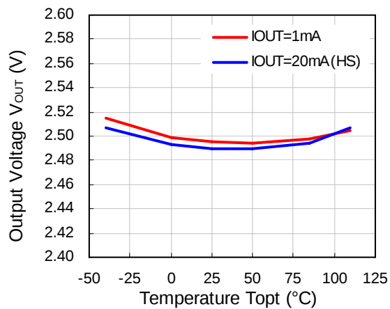
R1510S (VR=2.5V)
