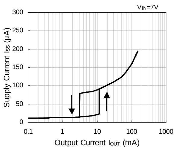
R1510SxxxA (VR=5.0V)
