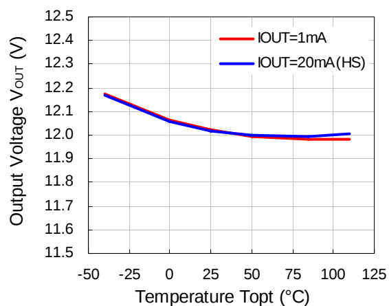
R1510S (VR=12.0V)
