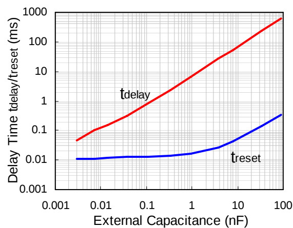
R1510SxxxC/D (VD=4.5V)
