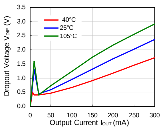
R1510S (VR=2.5V)
