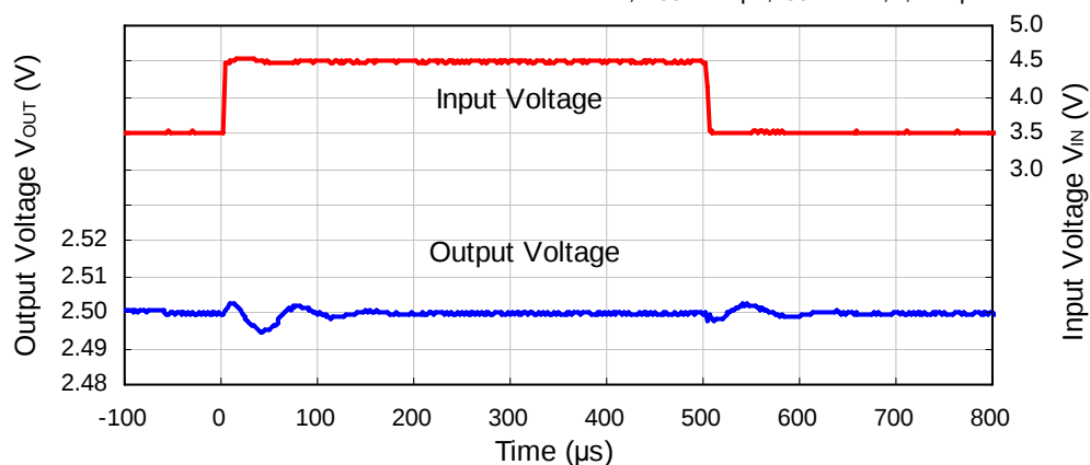
R1510S (VR=2.5V)
