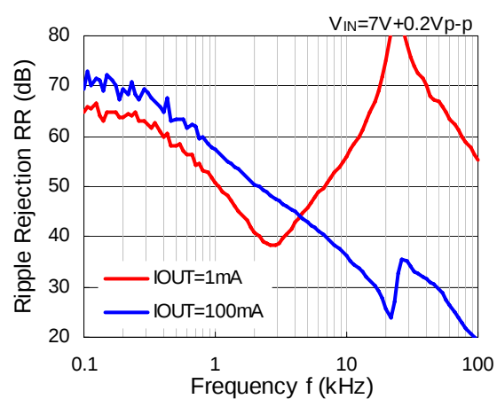
R1510S ( V_R=5.0V )
