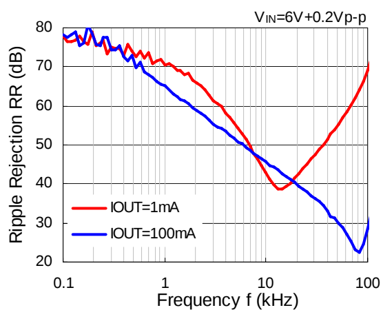
R1510S ( V_R=2.5V )
