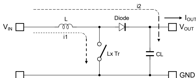
< Typical Circuit >
