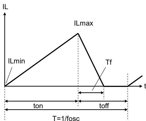
Discontinuous Mode
