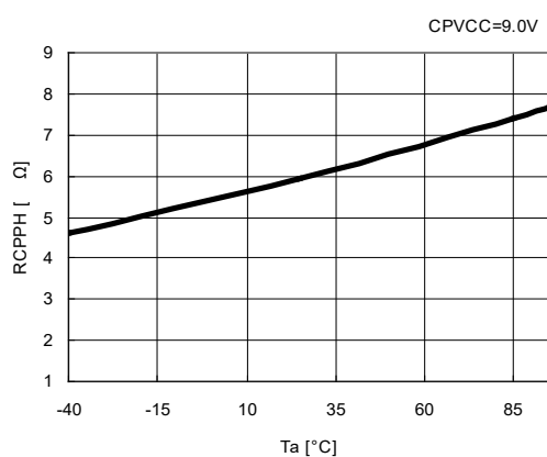
32) CPN"H"ON Resistance VS. Temperature R1290K102A
