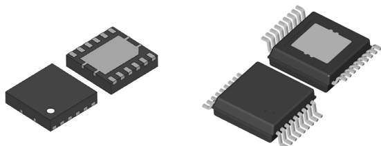
*Wettable Flanks DFN3030-12B 3.0 x 3.0 x 0.8 (mm)
