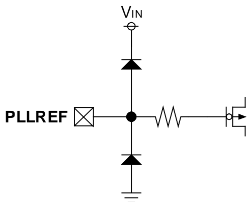
<PLLREF Pin>
