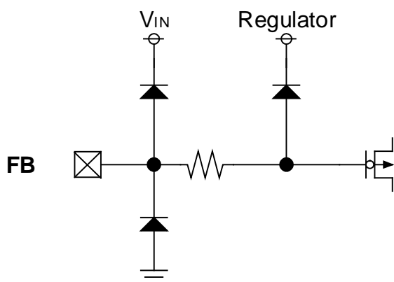
&lt;FB Pin&gt;
