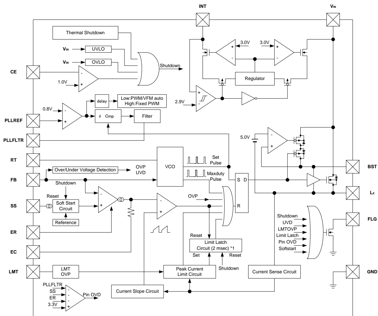
R1270S001A/B Block Diagram
