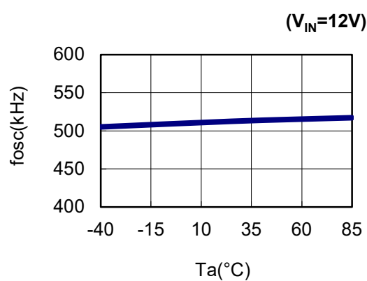
6) Oscillator Frequency(ver.E,F)
