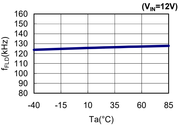
10) Fold-Back Frequency(ver.E,F)
