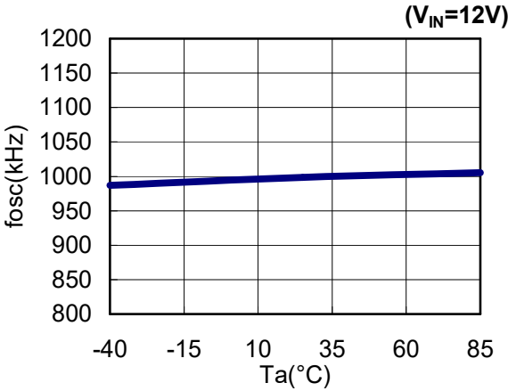
7) Oscillator Frequency(ver.G,H)
