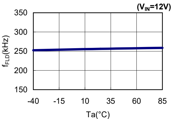
11) Fold-Back Frequency(ver.G,H)
