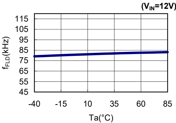
9) Fold-Back Frequency(ver.C,D)
