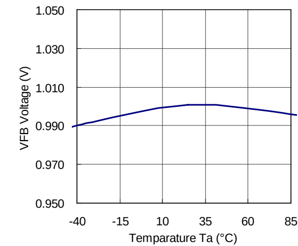
11) VFB Voltage vs. Temperature
