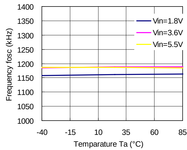
15) Oscillator Frequency vs. Temperature
