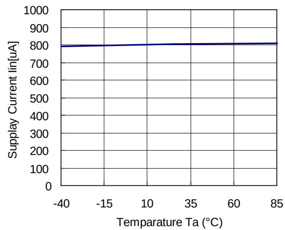
9) Supply Current vs. Temperature
