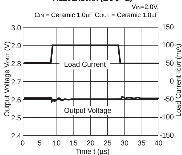
R1161x10xx (ECO=L)
