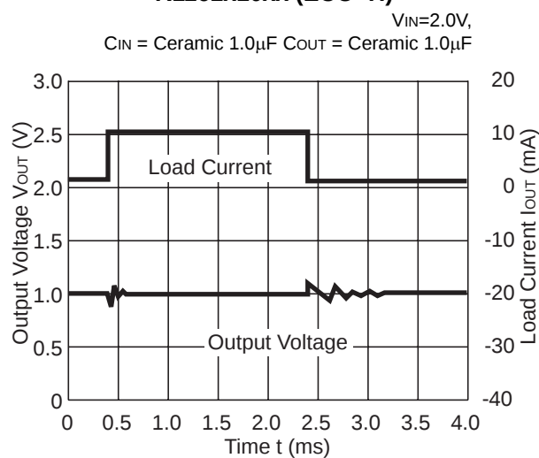
R1161x10xx (ECO=H)
