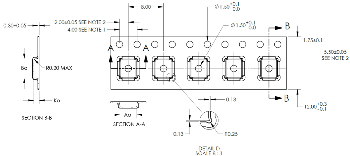
Figure 35: Tape specification
