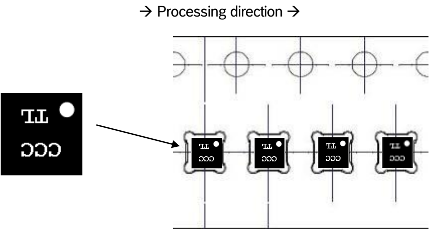
Figure 32: Orientation of the BMA223 devices relative to the tape
