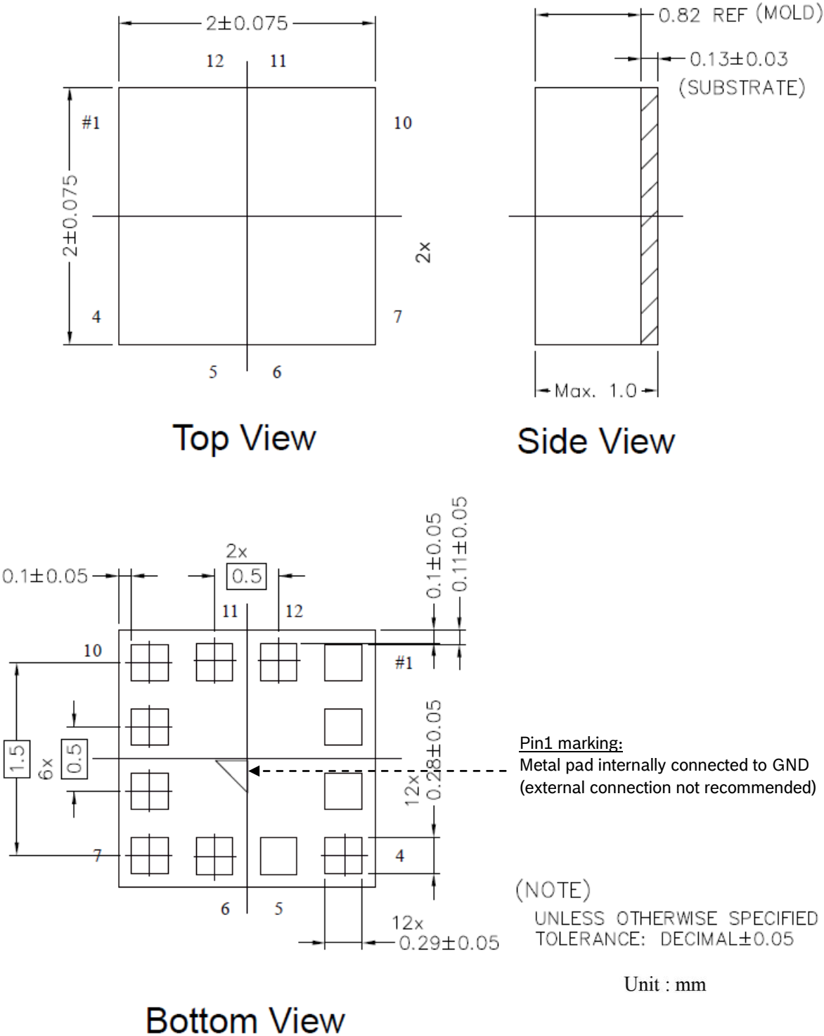
Figure 27: Package outline dimensions
