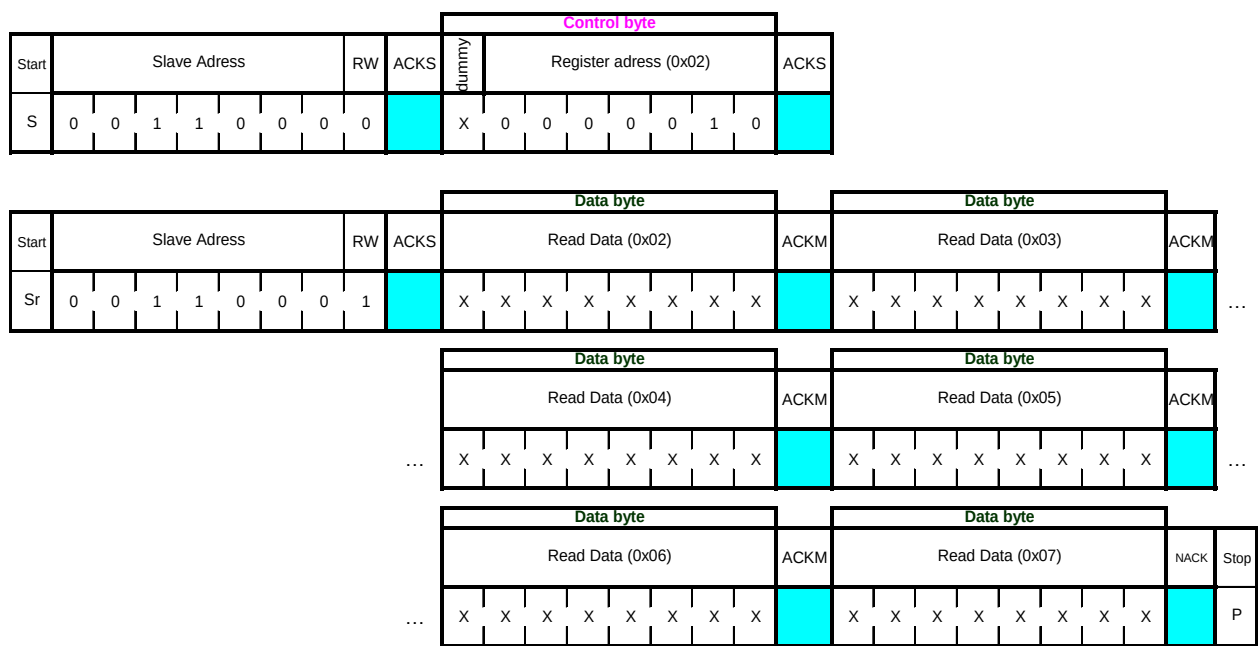
Figure 20: I²C multiple read
