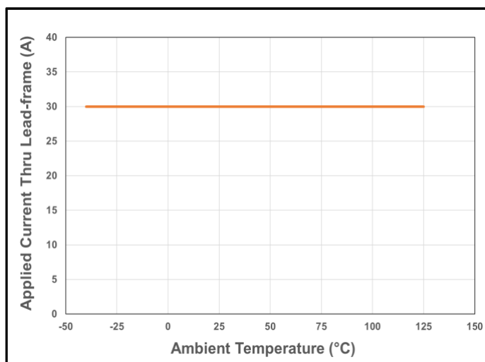
Figure 16. CT432 Current De-rating Curve for 30 A DC
