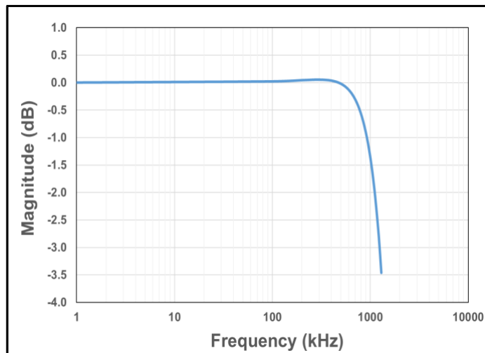
Figure 4. CT432 Bandwidth
