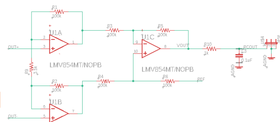
FIGURE 7 INSTRUMENTATION AMPLIFIER
