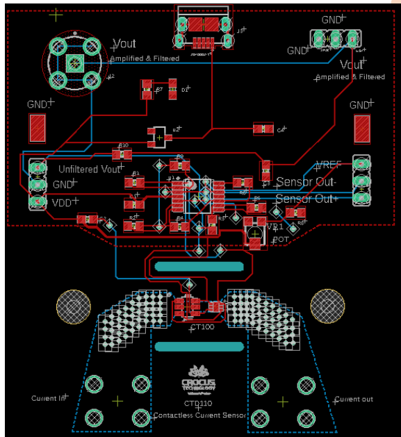
FIGURE 9 BOARD LAYOUT
