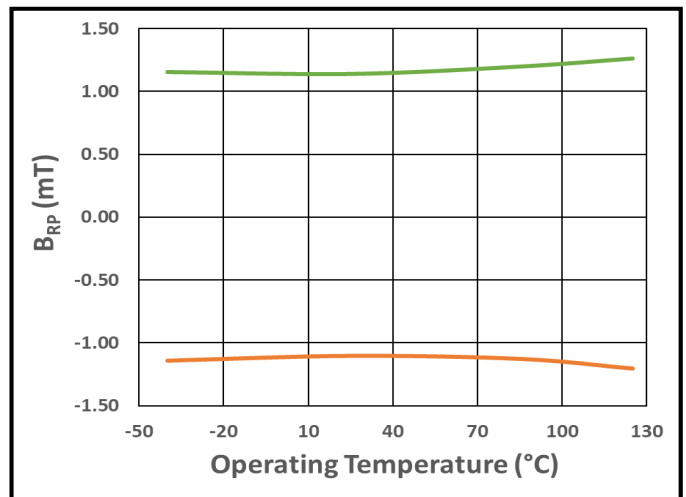
Figure 36. B_{RPN} (Orange) and B_{RPS} (Green) vs. Operating Temperature at V_{DD} = 3.0\text{ V}
