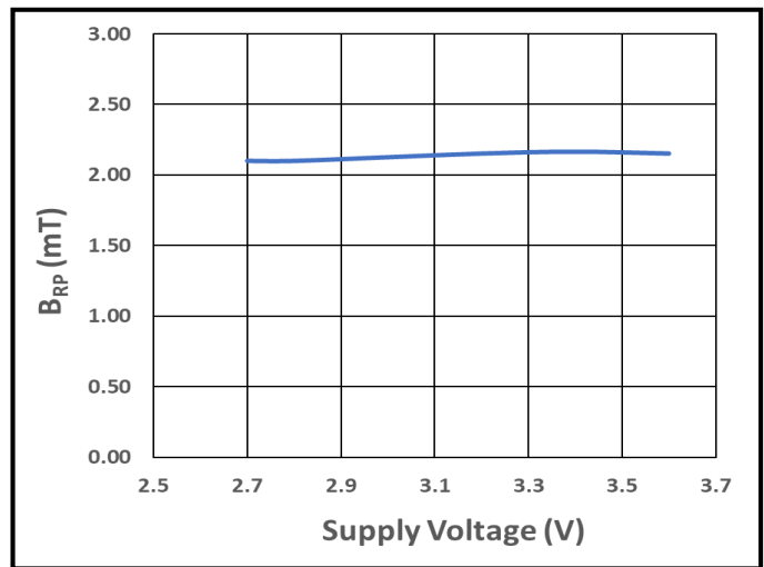
Figure 16. B_{RP} vs. Supply Voltage at +25^\circ\text{C}
