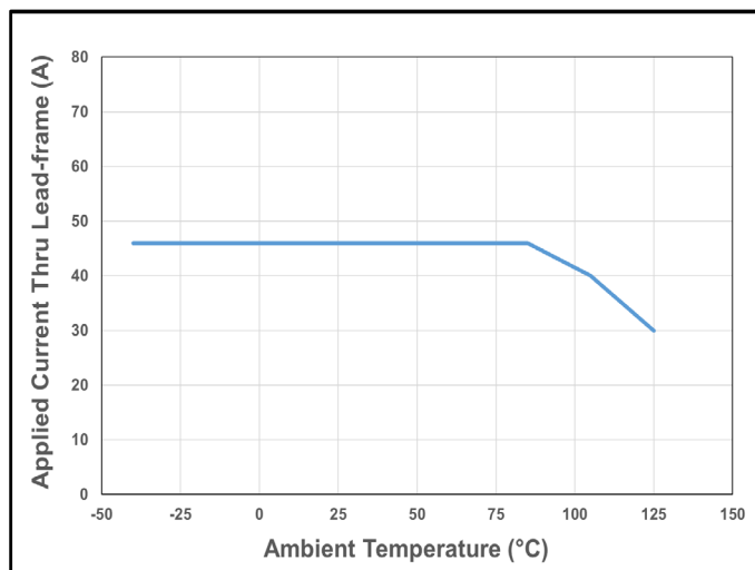
Figure 37. CT428 Current De-rating Curve for 65 A PK (46.0 A DC )
