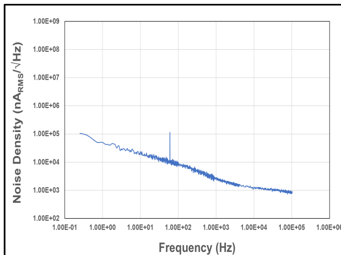
Figure 36. Noise Density vs. Frequency
