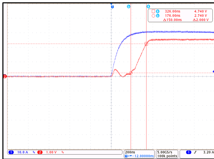
Figure 8. CT428 Rise Time; I_P = 30\text{ A}_{PK} and C_L = 100\text{ pF} (Blue = I_{LCC} , Red = V_{OUT} )
