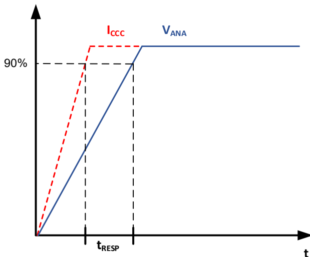
Figure 40. CT428 Response Time Curve
