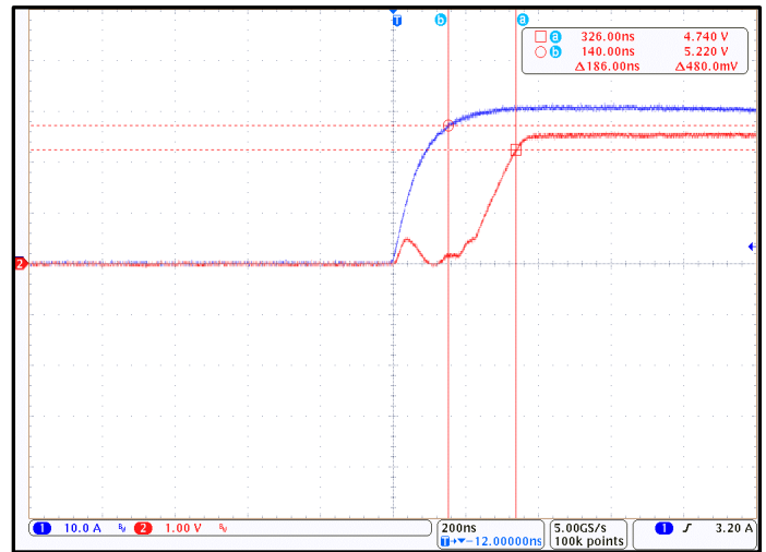
Figure 7. CT428 Response Time; I_P = 30\text{ A}_{PK} and C_L = 100\text{ pF} (Blue = I_{LCC} , Red = V_{OUT} )
