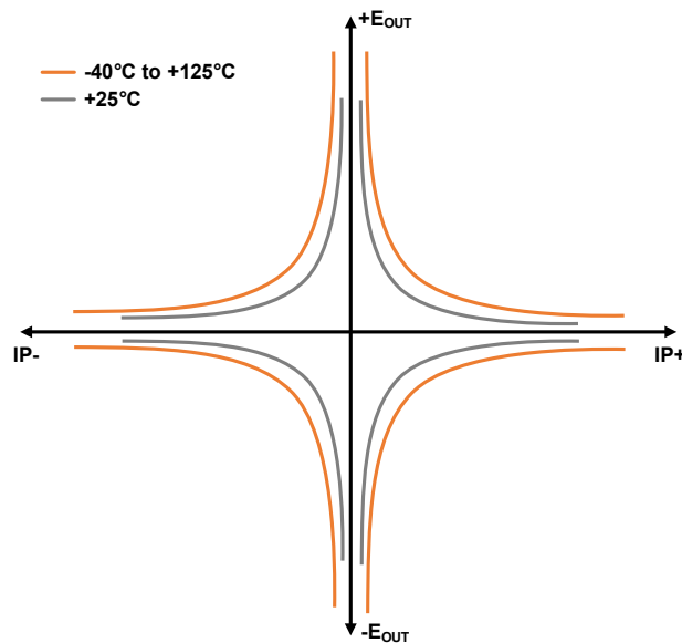
Figure 39. Total Output Error ( E_{OUT} ) vs. Sensed Current ( I_P )
