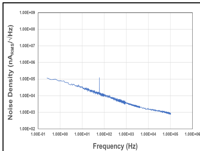
Figure 33. Noise Density vs. Frequency
