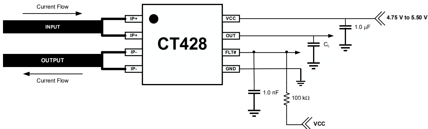
Figure 43. CT428 Application Block Diagram
