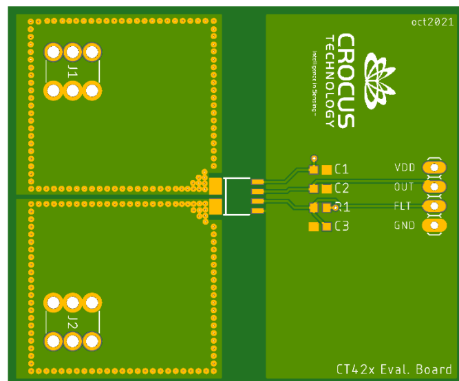
Figure 44. Recommended PCB Layout for the 20 A to 65 A variants of the CT428.
