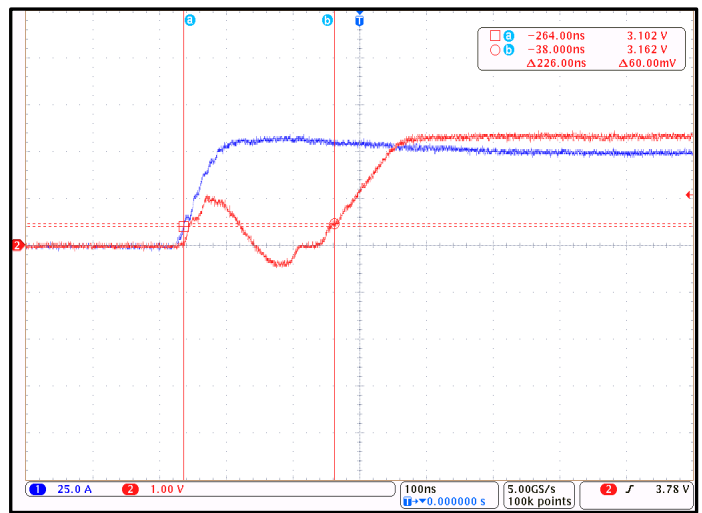
Figure 9. CT428 Propagation Delay; I_P = 30\text{ A}_{PK} and C_L = 100\text{ pF} (Blue = I_{LCC} , Red = V_{OUT} )
