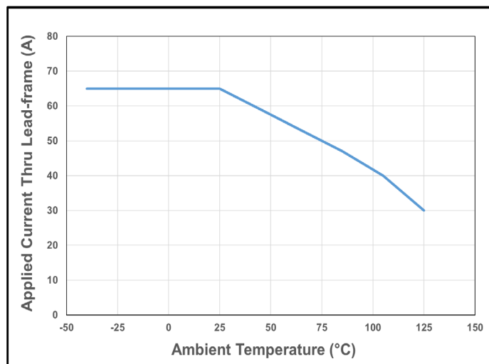
Figure 34. CT428 Current De-rating Curve for 65 A DC
