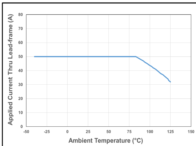
Figure 28. CT428 Current De-rating Curve for 50 A DC
