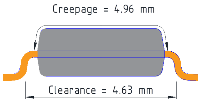
Figure 42. The Creepage and Clearance for the CT428's SOIC-8 package
