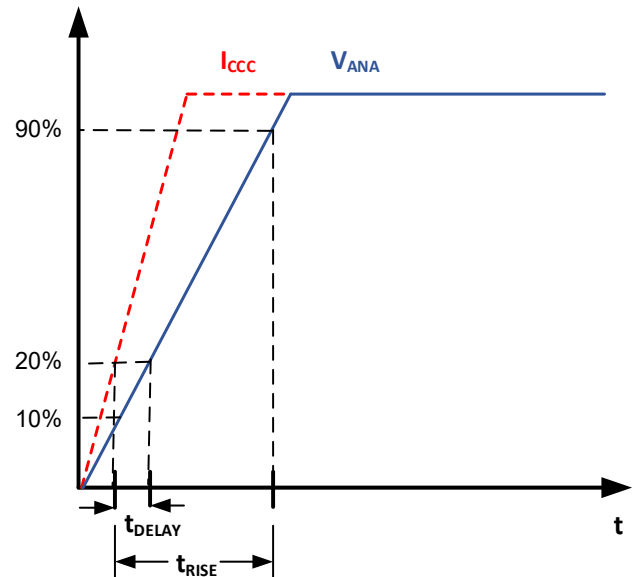
Figure 41. CT428 Propagation Delay and Rise Time Curve
