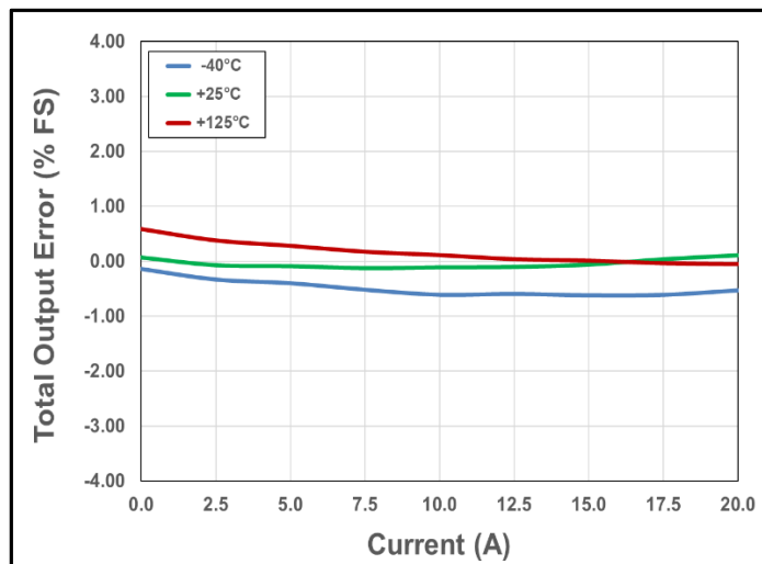
Figure 14. Total Output Error vs. Current vs. Temperature
