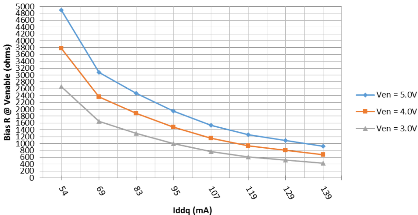
GRF4004 w/V dd = 5.0V: Required Bias R @ V enable vs. I ddq
