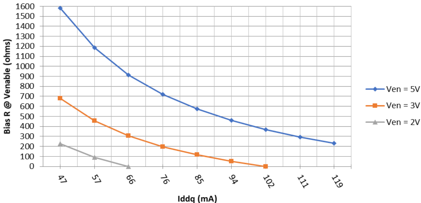
GRF2013 w/Vdd = 5.0V: Required Bias R @ Venable vs. Iddq
