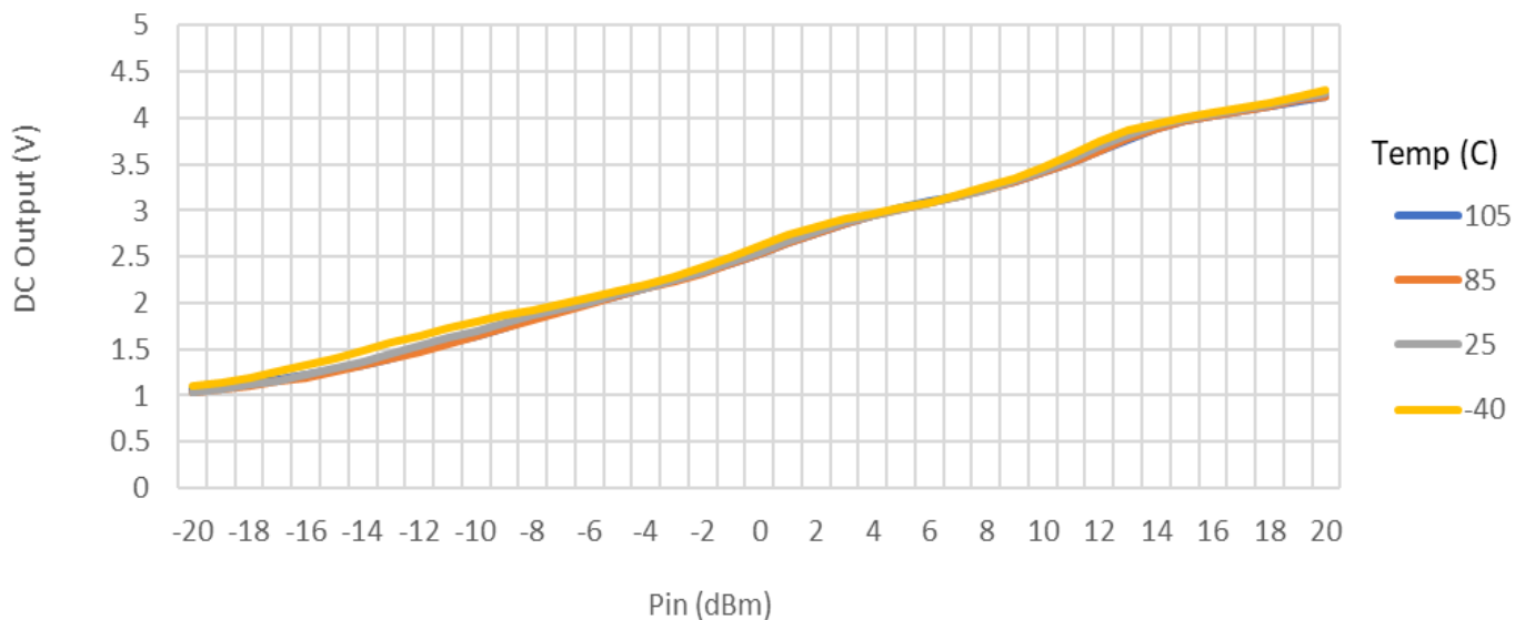
GRF1201 DC Output vs. RF Input Power over Temperature at 2.0 GHz; Vcc: 5.0 volts
