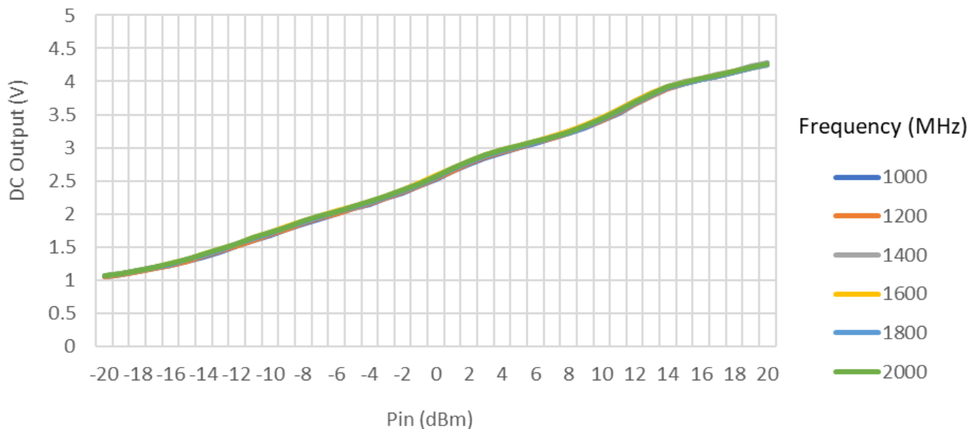
GRF1201 DC Output vs. RF Input Power over Frequency; Vcc: 5.0 volts
