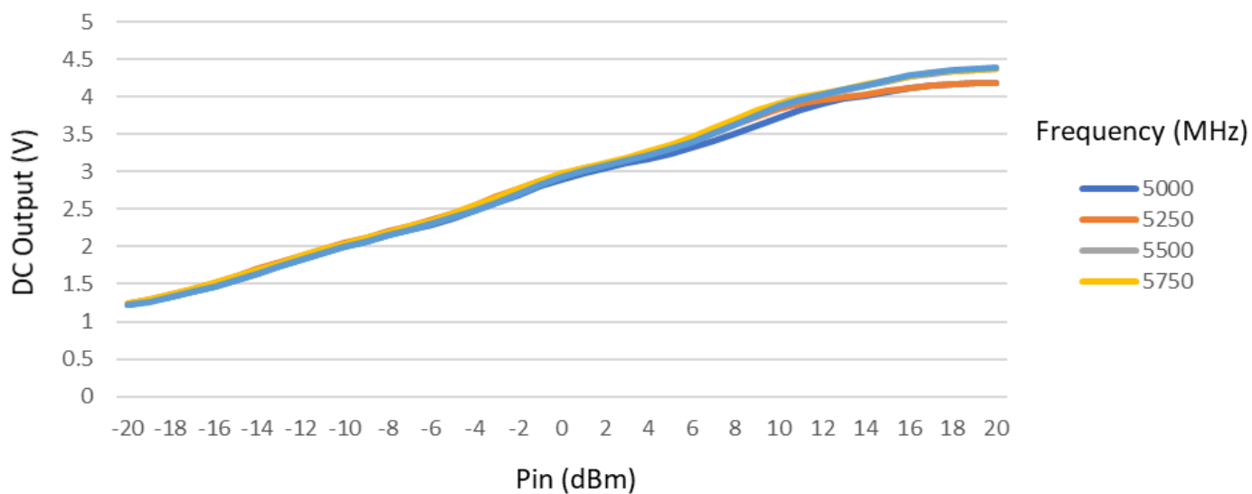
GRF1201 DC Output vs. RF Input Power over Frequency; Vcc: 5.0 volts
