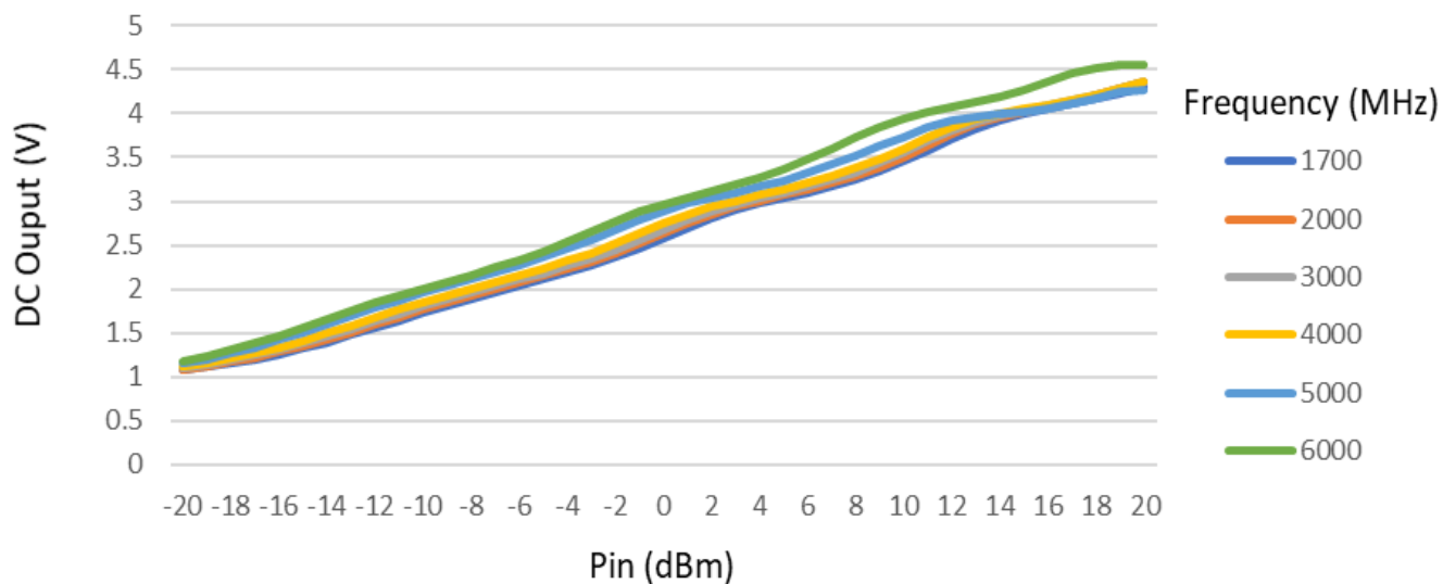
GRF1201 DC Output vs. RF Input Power over Frequency; Vcc: 5.0 volts
