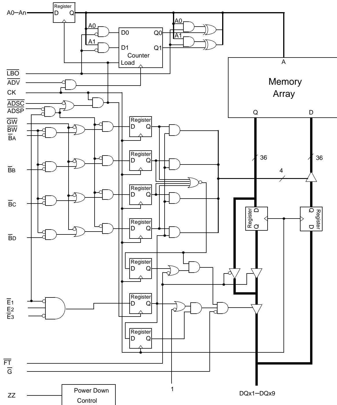
GS881E18/32/36C(T/D)-xxxIV Block Diagram
