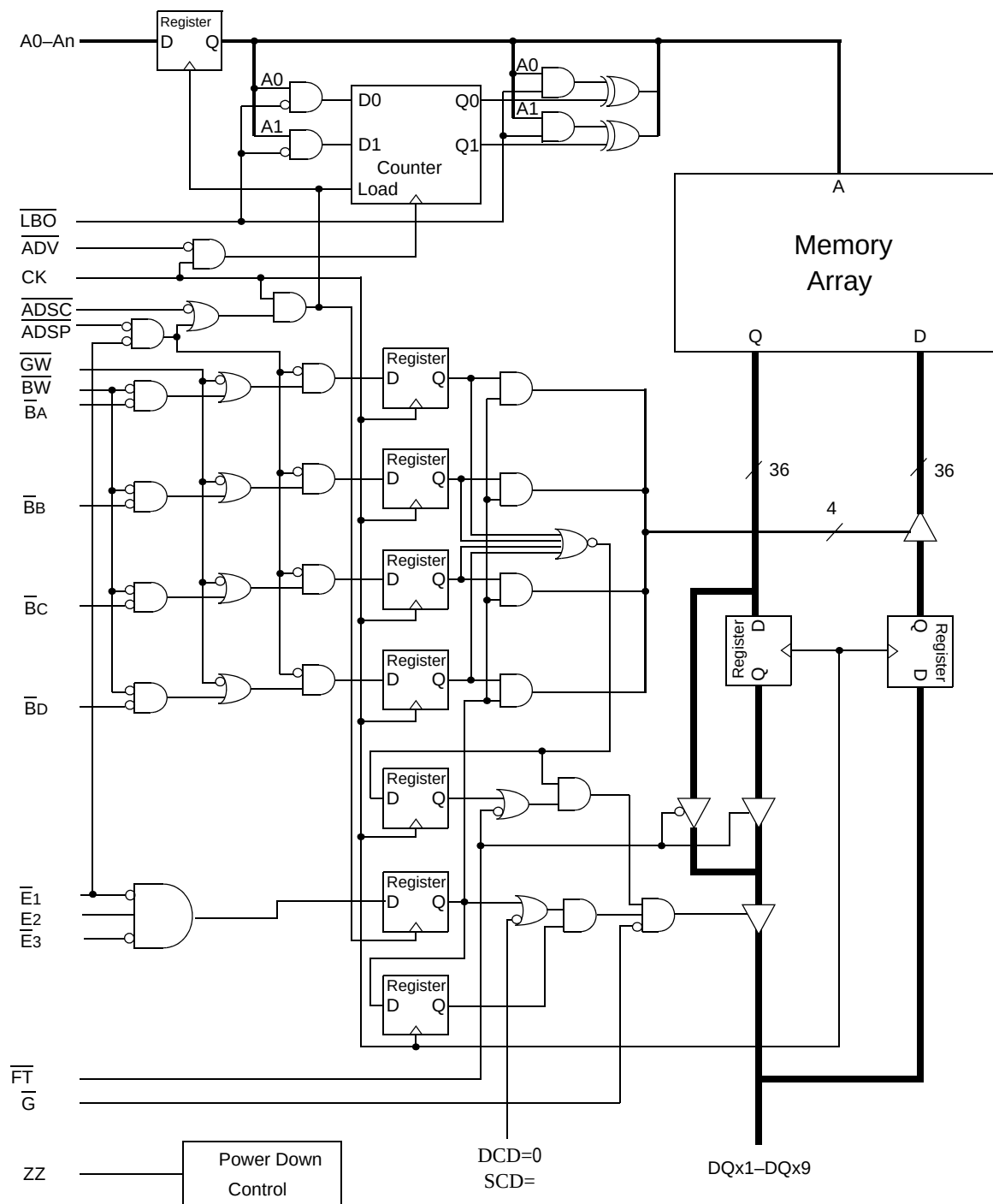
GS880E18/32/36CT-xxxIV Block Diagram
