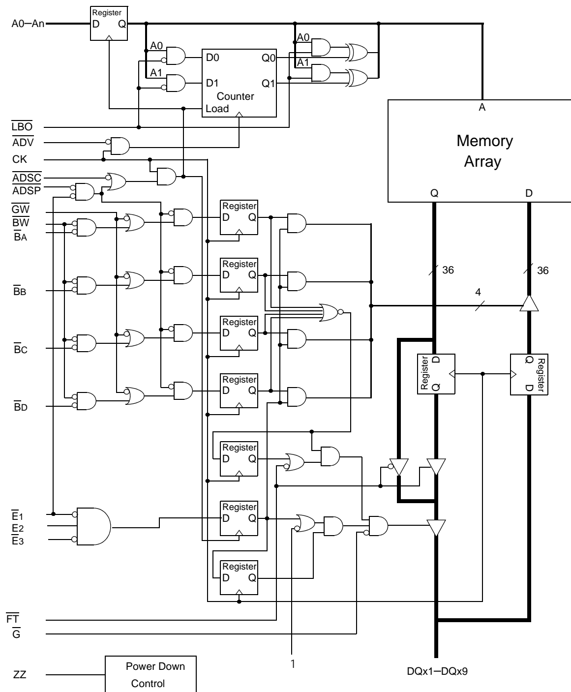
GS8161E18/32/36DGD-xxxV Block Diagram
