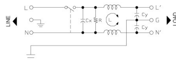
085- Electrical Schematic
