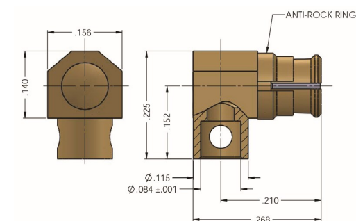
8676037G001-000 R/A Female RG 316 Cable
