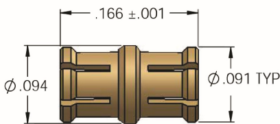
8828000G001 - 014 Female to Female “Bullet” Adapters Low Profile
