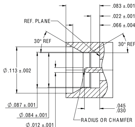
SMPM (Full Detent) Male PER MIL-STD-348A - Figure 328.2
