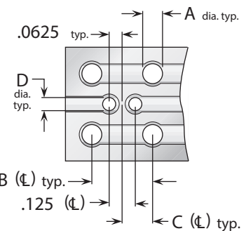
Twinax Connectors
