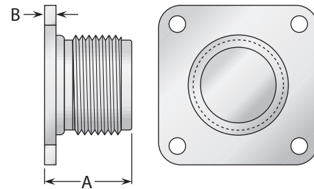
Figure 4 (Dummy receptacle)
