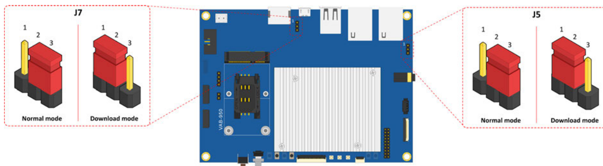
Figure 31: OS image jumpers diagram
