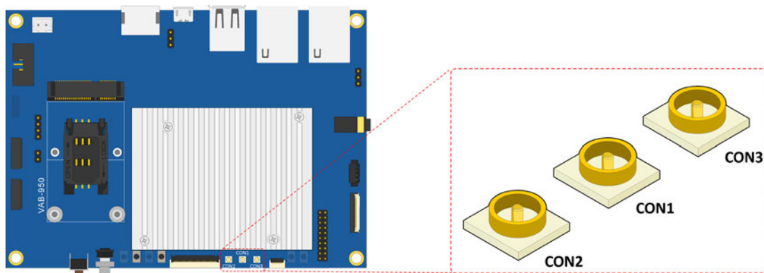
Figure 29: IPEX connectors diagram
